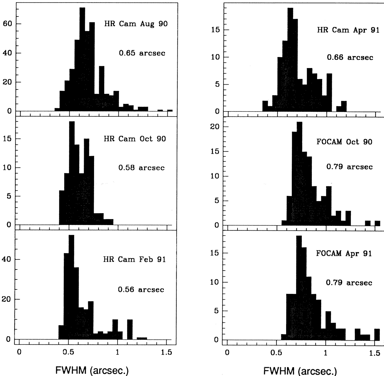
Figure 1: Statistics of image quality at CFHT for the period August 90 - April 91. Distributions of the FWHM of stellar profiles measured on images
