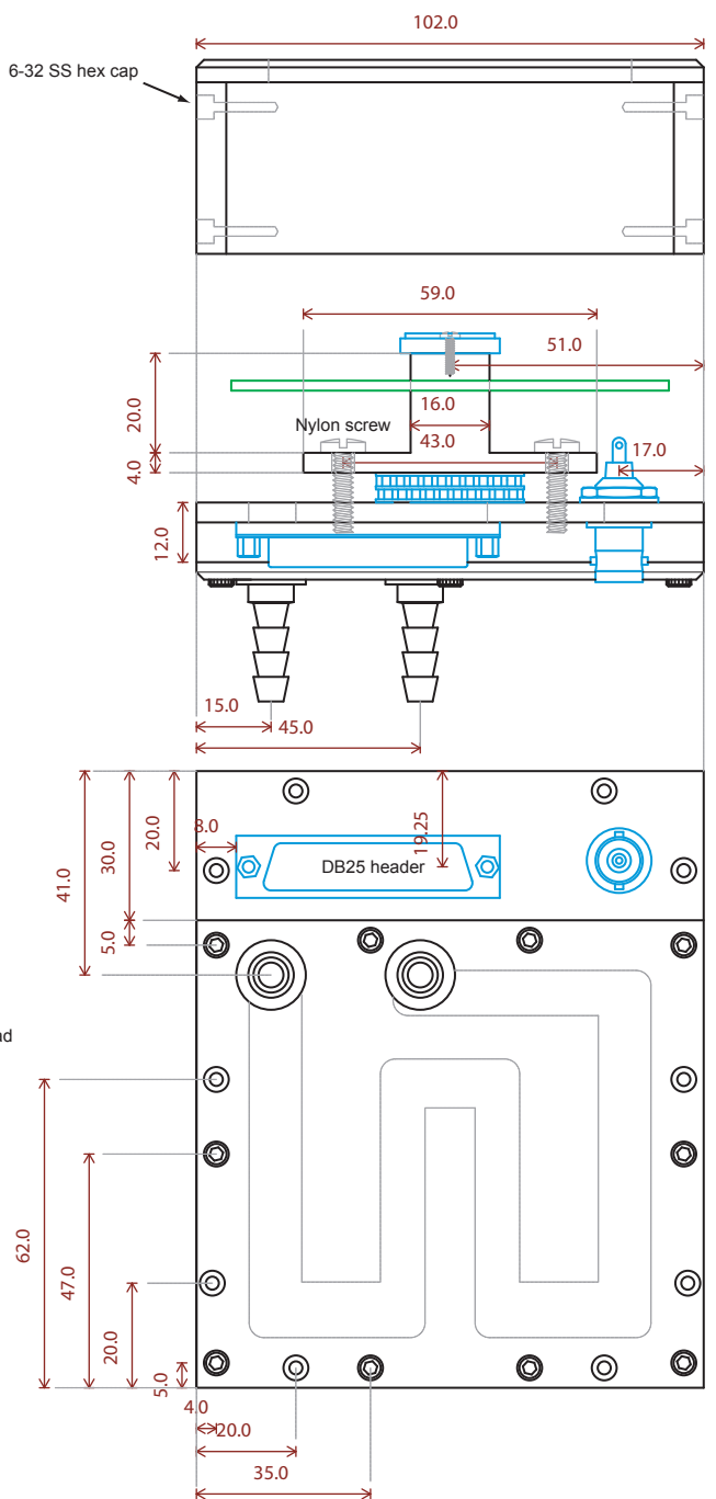
Pyxis camera housing Scale: 3/5 Dimensions: mm Material: Aluminum
